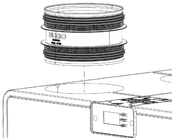
Push the connecting sleeve into the unit
