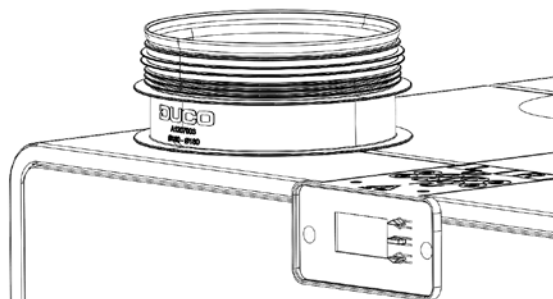
Push the connecting sleeve into the unit up to the stop flange
