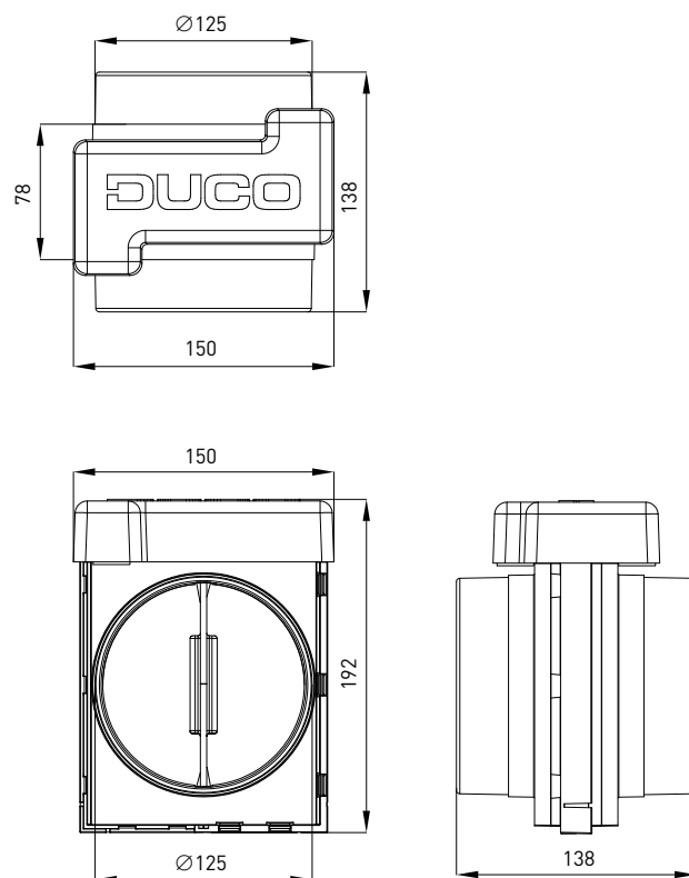
Multi-zone valve DucoBox Energy Comfort (Plus) Ø125
