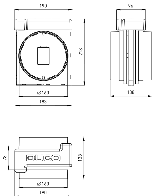
Multi-zone valve DucoBox Energy Comfort (Plus) Ø160
